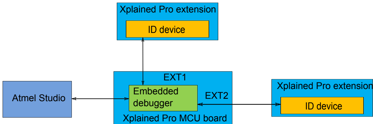
Figure 2-5 ID System Overview
